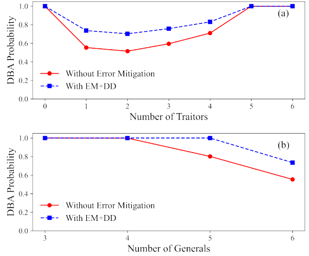
Figure 5. (a) Depicts the probability of achieving detectable broadcast with and without QEM and DD with a fixed network size n = 6 , and varying numbers of traitors present, while (b) depicts the probability of achieving detectable broadcast with and without QEM and DD in the presence of a single traitor with varying network size. 1000 iterations were performed for each data point, with a number of shots equal to 10,000. The trivial cases in (a) with a number of traitors m \in \{0, 5, 6\} are demonstrated clearly. In both (a) and (b) the significant performance improvement with the utilization of QEM and DD is visible over the unmitigated case with greater success probability in every non-trivial case.
